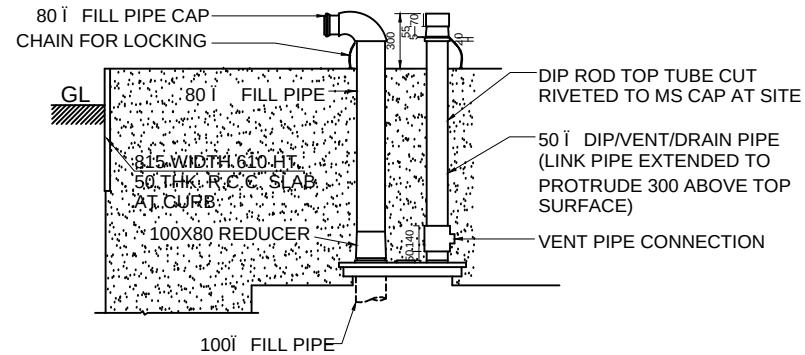
DETAILS AT 'C'
